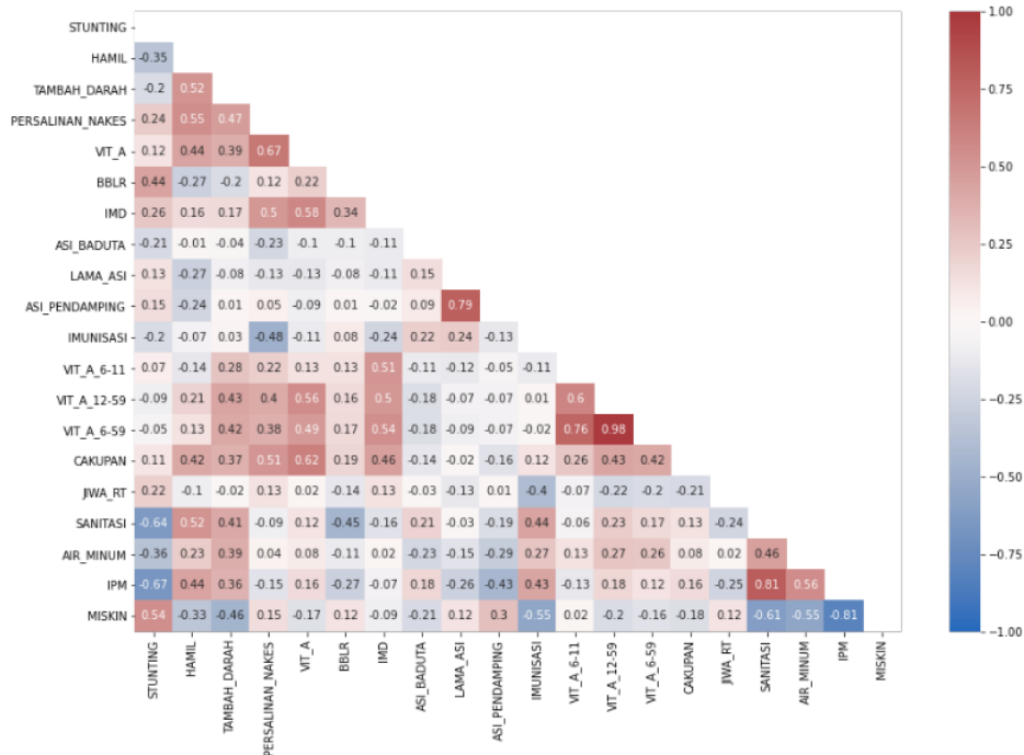
Figure 4. Feature Correlation Value
