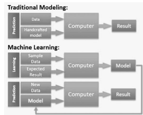
Figure 1. Traditional Modeling and Machine Learning Differences
