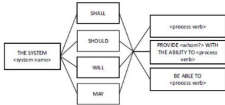
Gambar 1. Pola Requirement Boilerplate (Pohl and Rupp, 2015).
