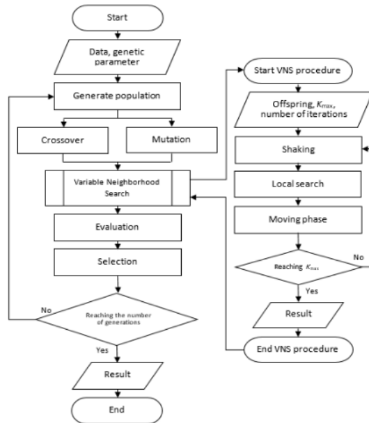
Fig. 1. Scheme of GA-VNS
