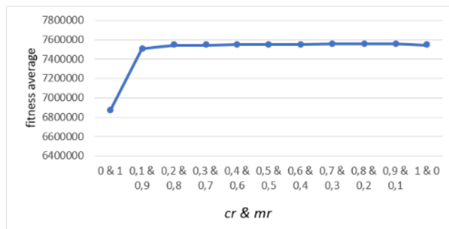
Fig. 7. Combination of cr and mr Testing
