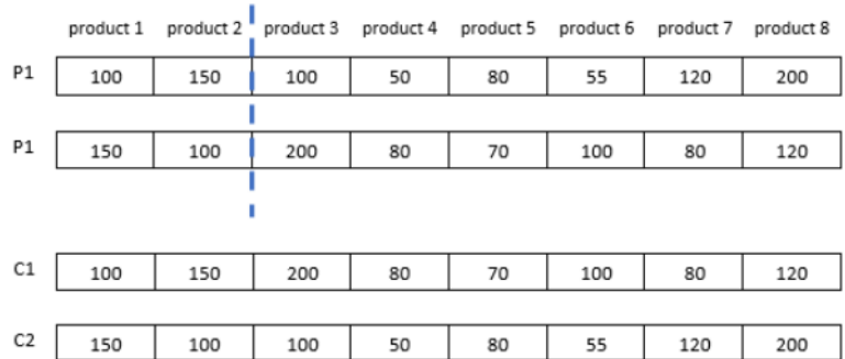
Fig. 3. Crossover
