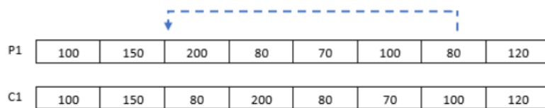
Fig. 3. Crossover
