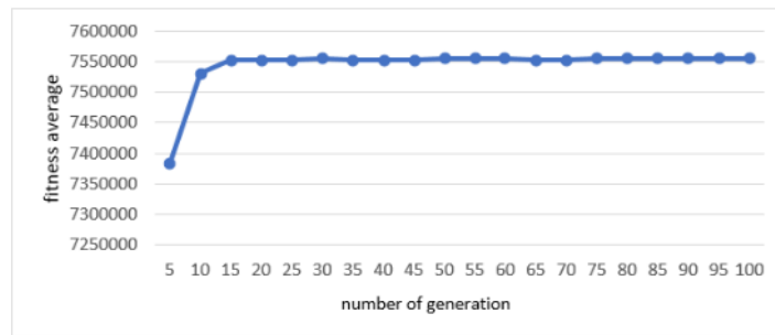
Fig. 6. Generations Number Testing
