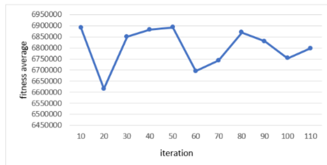
Fig. 9. Iteration Testing
