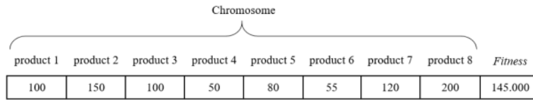
Fig. 2. Chromosome representation
