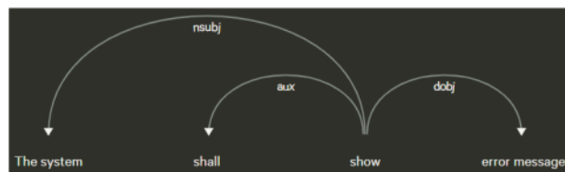
Figure 8. Word Dependency Parsing by SpaCy NLP Illustration
