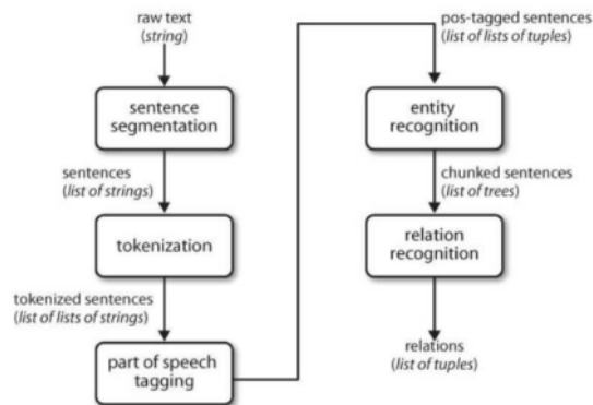
Figure 3. NLP Process Pipeline for Information Retrieval from Text Document [31]
