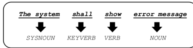
Figure 7. POS Tagging Illustration
