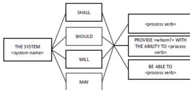
Figure 1. Requirements Boilerplate Template
