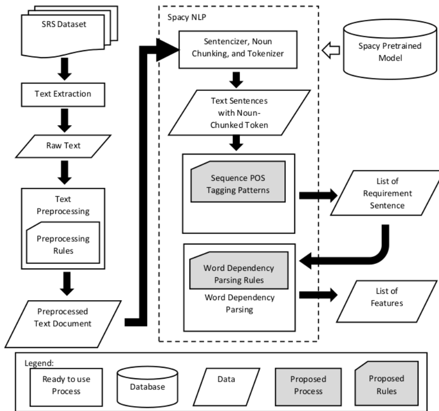
Figure 5. Feature Extraction Automation Framework from SRS Document
