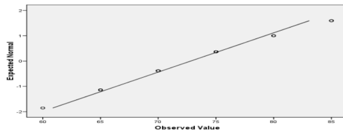
Figure 6 Normal QQ Plot for Concept Applications in PBL Learning Strategies
